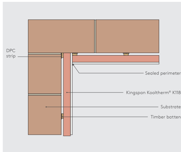
Figure 10 - Internal Corner Detail
