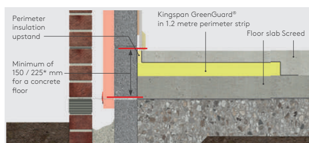
Figure 2 - Perimeter Strip Concrete Floor Insulation
