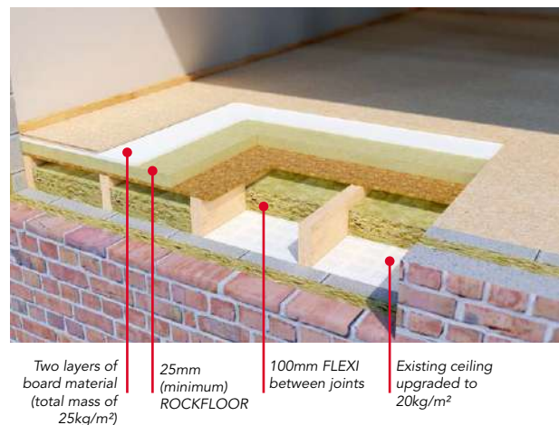
Figure 11 Separating floors
