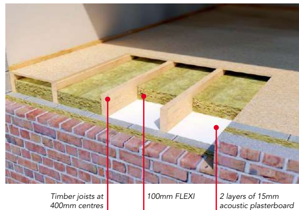
Figure 10 Internal floors
